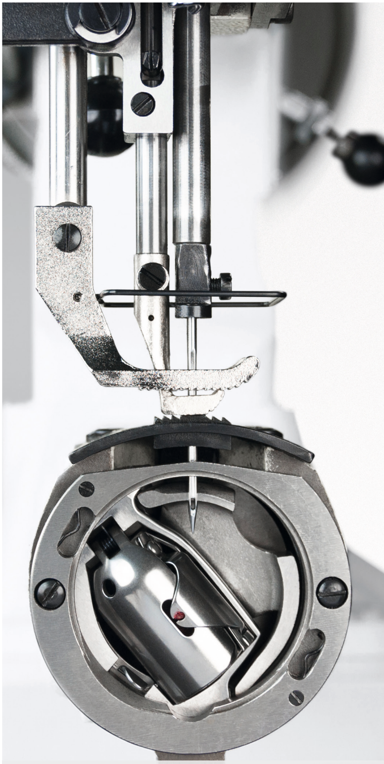
Barrel hook for extra heavy-duty applications. Thread sizes up to 8/3.
